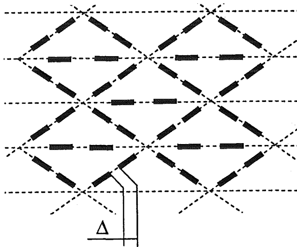
FIG.11. Crack array of infinitesimal crack density, \rho \rightarrow 0 that reduces the effective stiffness to zero. Note that this effect is achieved without creating a line of cracks crossing the representative area - the array is dense everywhere (since H \rightarrow 0 ).
