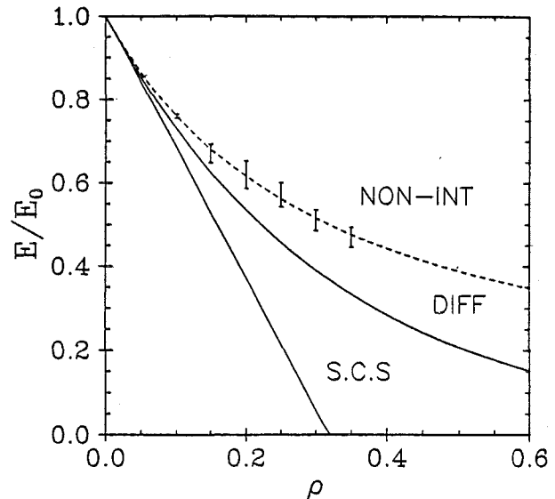
FIG.8. Effective Young's modulus, randomly oriented cracks: results for sample arrays vs predictions of the approximation of non-interacting cracks, self-consistent and differential schemes.
