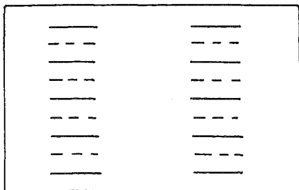
Fig.12. Introduction of new cracks (dashed lines) reduces the SIFs and, at the same time, produces elastic "softening"
