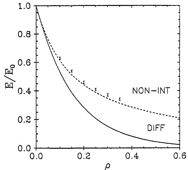
FIG.9. Effective Young's modulus, parallel cracks: results for sample arrays vs the approximation of non-interacting cracks and the differential scheme.
