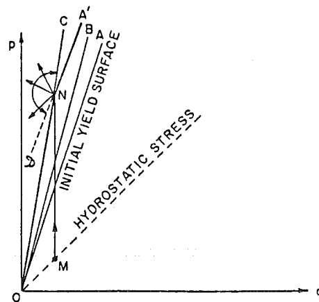
FIG.3. Range of path-independence (cone CD) and formation of a vertex on the loading surface in axisymmetrical compression; NA' is parallel to the initial loading surface OA most favourably oriented crack. MN shows the loading path (axial compression at constant lateral stress).
