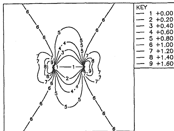
FIG.5. Zones of shielding and amplification of the stress component \sigma_{yy} generated by a crack subjected to a uniform tension (lines of equal level are indicated). The shielding zone is less intense but larger than the amplification zone.
