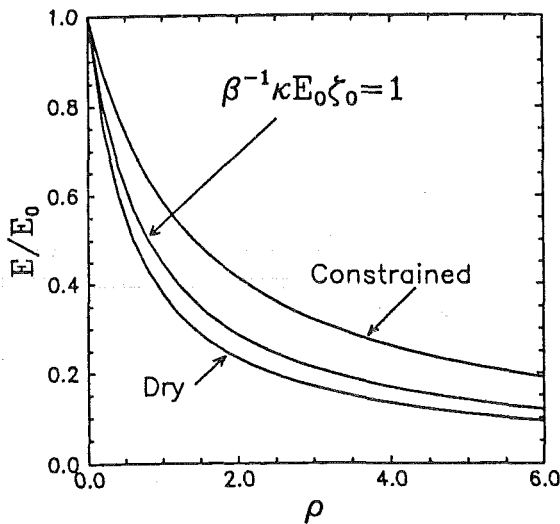
FIG.4. Young's modulus of a solid with fluid-filled cracks as a function of crack density, at various values of \kappa E_0 \zeta_0 . Note a gradual transition from the "dry" cracks curve to the curve for cracks constrained against opening.
