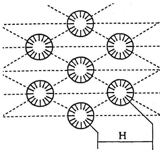
FIG.10. Crack array of infinite crack density, \rho \rightarrow \infty producing an infinitesimal impact on the effective moduli.
