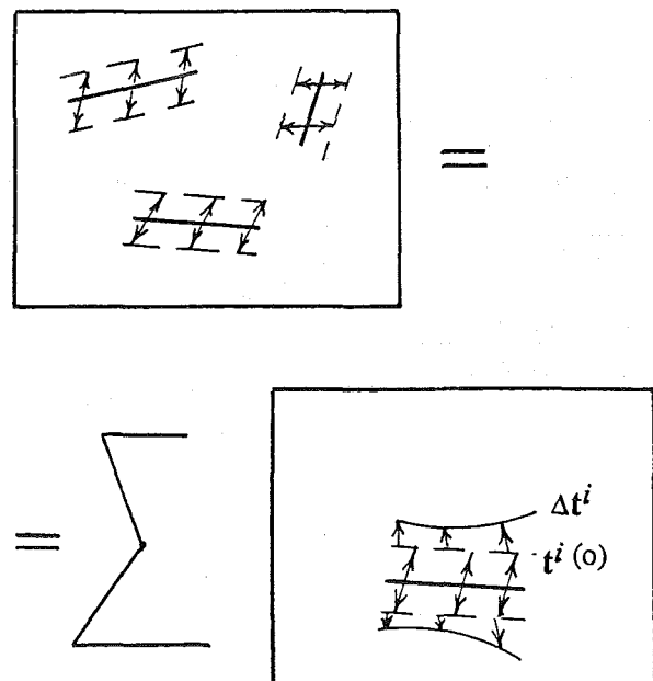
FIG.6. Stress superpositions. Traction \Delta \mathbf{t}^i(\xi^i) , induced on the i -th crack by the other cracks, accounts for interactions; it may either increase or reduce \mathbf{t}^i . If crack locations are random (and tractions are prescribed on the boundary), the average of \langle \Delta \mathbf{t}^i \rangle over the array is zero - there is no impact of interactions on the effective moduli.
