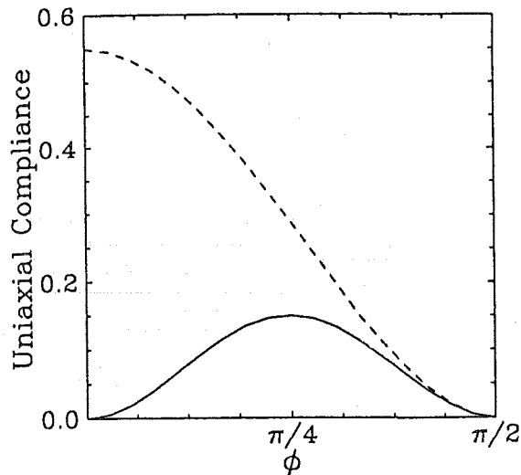
FIG.2. Uniaxial compliance (additional, due to cracks) of a 2-D solid with parallel cracks, as a function of direction of loading (forming angle \phi with a normal to cracks (normalized to \pi p \sigma / E_0 ). Solid and dashed lines indicate constrained and unconstrained cracks. Imposition of the constraint shifts the direction of maximal compliance by 45^\circ and sharply reduces strains. This illustrates the difference between responses to compression and tension.
